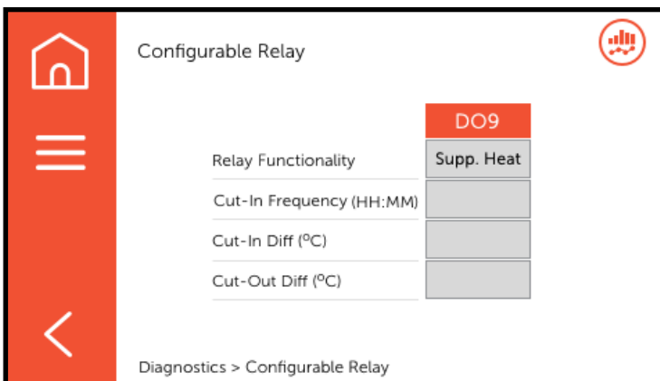
Fig 21 Diagnostics—Configurable Relay Menu (Supplementary Heating)
